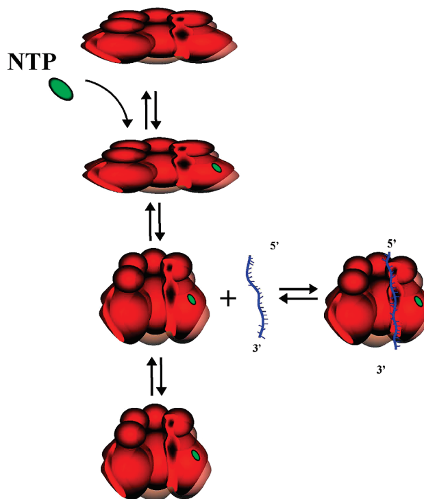
FIGURE 8: Schematic model of the sequential kinetic mechanism of the NTP binding to the single, noninteracting nucleotide-binding site of the RepA hexamer and the selection of the intermediates of the reaction by the ssDNA, based on the data obtained in this work. Initially, all six nucleotide-binding sites are independent and equivalent (13, 14). The single NTP molecule binds to an independent nucleotide-binding site forming the (H-N) 1 intermediate (13, 14). The (H-N) 1 intermediate has a modestly increased affinity for the nucleic acid bound in the outer DNA-binding site of the enzyme (56). Nevertheless, (H-N) 1 is short-lived. The subsequent transition to the (H-N) 2 intermediate is fast and energetically very favorable. The (H-N) 2 intermediate is preferentially selected by the single-stranded conformation of the DNA and dominates the fractional distribution of the RepA-cofactor-ssDNA ternary complex in the equilibrium state. Only a small fraction of the formed complex transforms into the (H-N) 3 intermediate (details in the text).
