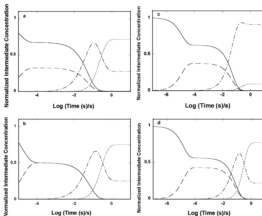
FIGURE 7: (a) Computer simulation of the time course of the fractional concentration distribution of different TNP-ATP intermediates, in the binding to the RepA hexamer helicase, using the determined rate constants included in Table 1, in buffer T5, containing 5 mM \text{MgCl}_2 , at 10 °C. (b) Analogous plots of the fractional concentration distributions of different TNP-ADP intermediates, in the binding to the RepA helicase, using the determined rate constants included in Table 1, at 10 °C. (c) Computer simulation of the time course of the fractional concentration distribution of different TNP-ATP intermediates, in the binding to the RepA hexamer helicase, using the determined rate constants included in Table 1, in buffer T5 (10 °C), containing 5 mM \text{MgCl}_2 and 7 \times 10^{-5} M (oligomer) ssDNA 20-mer, dT(pT) 19 . (d) Computer simulation of the time course of the fractional concentration distribution of different TNP-ADP intermediates, in the binding to the RepA helicase, using the determined rate constants included in Table 1, in buffer T5 (10 °C), containing 5 mM \text{MgCl}_2 and 7 \times 10^{-5} M (oligomer) ssDNA 20-mer, dT(pT) 19 . The selected total nucleotide cofactor concentration is 1 \times 10^{-7} M. The selected RepA helicase concentration is 1 \times 10^{-4} (protomer): free nucleotide cofactor (—), (H–N) 1 (— —), (H–N) 2 (— — —), and (H–N) 3 (— — — —). The bimolecular step is modeled close to the diffusion-controlled reaction with a k_1 of 1 \times 10^6 \text{ M}^{-1} and the k_{-1} adjusted to give the experimentally obtained partial equilibrium constant, K_1 = k_1/k_{-1} (details in the text).
