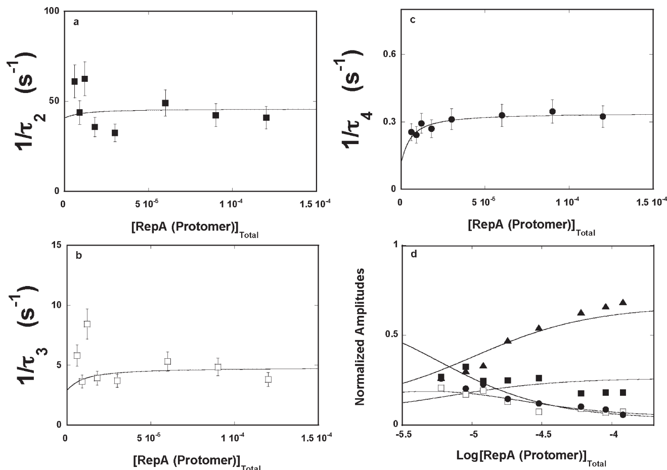
FIGURE 4: Dependence of the reciprocal relaxation times for the binding of TNP-ATP to the RepA helicase in buffer T5 (10 °C), in the absence of magnesium, on the total concentration of the enzyme (protomer): (a) 1/\tau_2 (■), (b) 1/\tau_3 (□), and (c) 1/\tau_4 (●). (d) Dependence of the individual normalized relaxation amplitudes A_1 (▲), A_2 (■), A_3 (□), and A_4 (●) of the kinetic process of binding of TNP-ATP to the RepA helicase in buffer T5 (10 °C), in the absence of magnesium, on the logarithm of the total concentration of the enzyme (protomer). The solid lines in panels a–d are nonlinear least-squares fits of the experimental data to the four-step sequential mechanism, defined by eq 9. The obtained kinetic and spectroscopic parameters are included in Table 2 (details in the text). The error bars are standard deviations obtained from three or four independent experiments.
