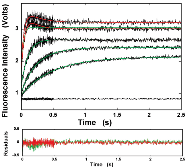
FIGURE 2: Fluorescence stopped-flow kinetic traces (top), recorded in two time bases, 0.5 and 2.0 s, after the RepA helicase had been mixed with TNP-ATP in buffer T5, containing 5 mM MgCl 2 ( \lambda_{\text{ex}} = 408 nm, and \lambda_{\text{em}} > 500 nm). The final concentrations of the RepA helicase (protomer) are, from the top, 12 \times 10^{-5} , 9 \times 10^{-5} , 3 \times 10^{-5} , 1.2 \times 10^{-5} , and 0.6 \times 10^{-5} M. The final concentration of the nucleotide is 5 \times 10^{-7} M. The solid green and red lines are the single-exponential and double-exponential, nonlinear least-squares fits, respectively, of the experimental curves, using eq 3. The bottom panel shows the deviations of the experimental curve from the fit using the single-exponential (green) and double-exponential functions (red) for the sample containing 9 \times 10^{-5} M (protomer) RepA helicase.
