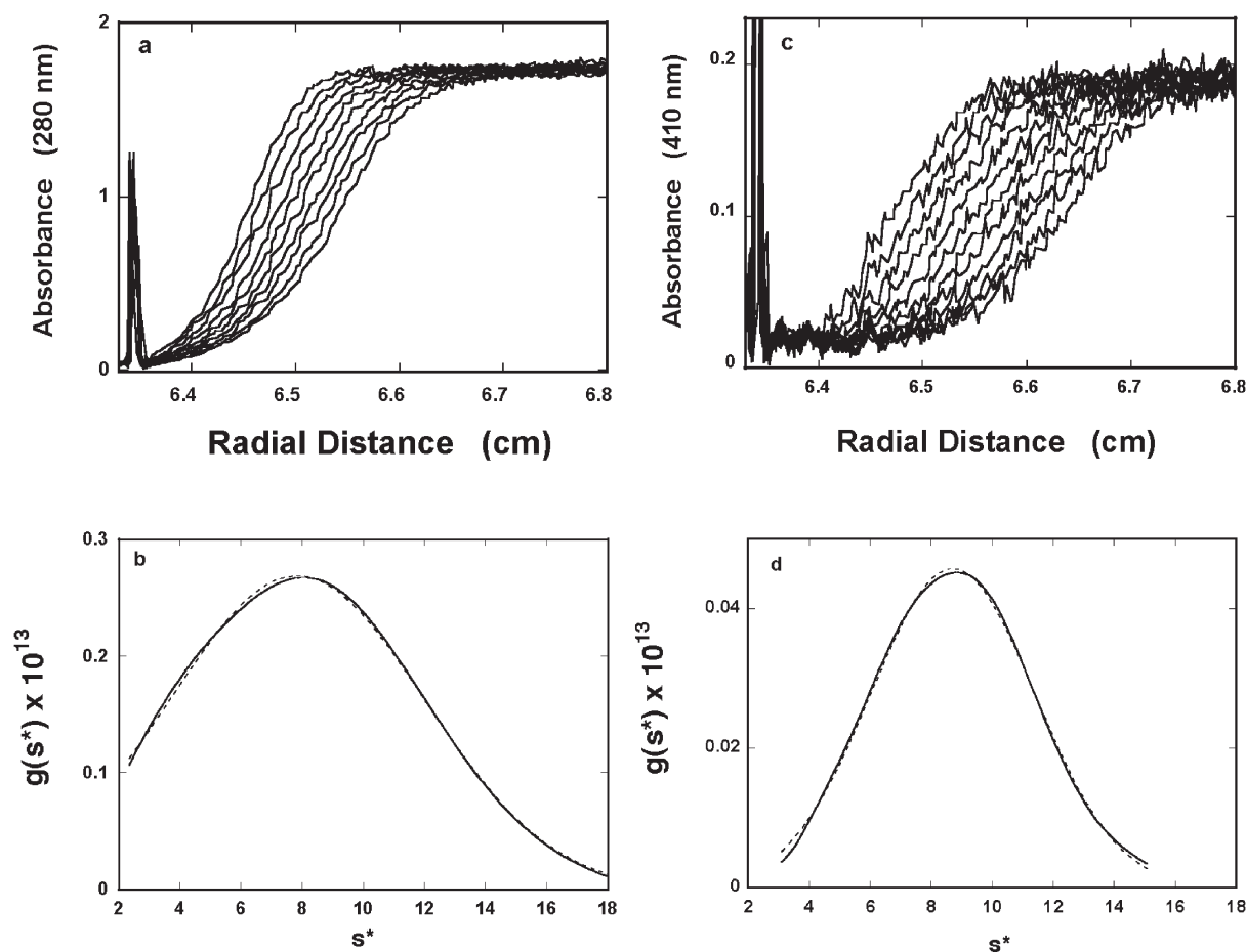
FIGURE 5: (a) Absorption profiles, recorded at 280 nm, of analytical sedimentation velocity runs of the RepA helicase alone, in buffer T5 (pH 7.6 and 10 °C), in the absence of magnesium. The total protein concentration is 1 \times 10^{-5} M (hexamer). (b) The solid line is the apparent average sedimentation coefficient distribution g(s^*) , as a function of the radial sedimentation coefficient coordinate, s^* , obtained from time derivatives of the RepA sedimentation profiles recorded at 280 nm, in buffer T5 (pH 7.6 and 10 °C), in the absence of magnesium (35000 rpm). The dashed line is the nonlinear least-squares fit of the experimental distribution using the time-derivative method. Both plots are corrected for the solution conditions (details in the text). (c) Absorption profiles, recorded at 410 nm, of analytical sedimentation velocity runs of the RepA helicase–TNP-ADP complex, in buffer T5 (pH 7.6 and 10 °C), in the absence of magnesium. The total protein and cofactor concentrations are 1 \times 10^{-5} M (hexamer) and 6.5 \times 10^{-6} M, respectively. (d) The solid line is the apparent average sedimentation coefficient distribution, g(s^*) , as a function of the radial sedimentation coefficient coordinate, s , obtained from time derivatives of sedimentation profiles of the RepA–TNP-ADP complex recorded at 410 nm, in buffer T5 (pH 7.6 and 10 °C), in the absence of magnesium (35000 rpm). The dashed line is the nonlinear least-squares fit of the experimental distribution using the time-derivative method. Both plots are corrected for the solution conditions (details in the text).
