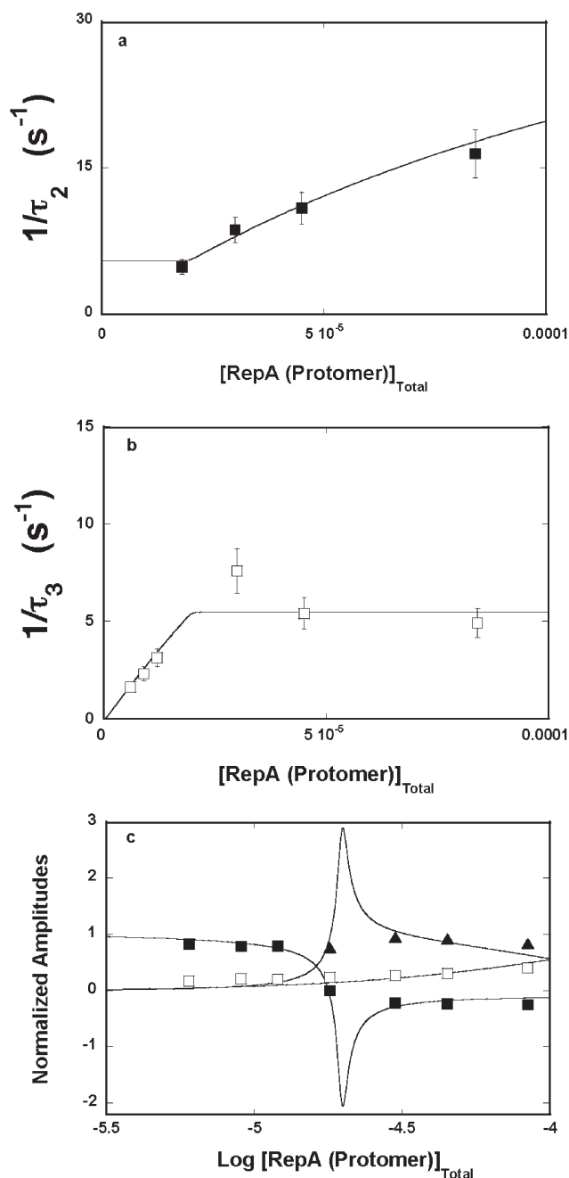
FIGURE 6: Dependence of the reciprocal relaxation times for the binding of TNP-ATP to the RepA helicase in buffer T5 (10 °C), containing 5 mM MgCl 2 and 7 \times 10^{-5} M (oligomer) ssDNA 20-mer, dT(pT) 19 , on the total concentration of the enzyme (protomer): (a) 1/\tau_2 (■) and (b) 1/\tau_3 (□). (c) Dependence of the individual normalized relaxation amplitudes, A_1 (▲), A_2 (■), and A_3 (□), of the kinetic process of binding of TNP-ADP to the RepA helicase in buffer T5 (10 °C), containing 5 mM MgCl 2 and 7 \times 10^{-5} M (oligomer) ssDNA 20-mer, dT(pT) 19 , on the logarithm of the total concentration of the enzyme (protomer). The solid lines in panels a–c are nonlinear least-squares fits of the experimental data to the three-step sequential mechanism, defined by eq 5. The obtained kinetic and spectroscopic parameters are included in Table 1 (details in the text). The error bars are standard deviations obtained from three or four independent experiments.
