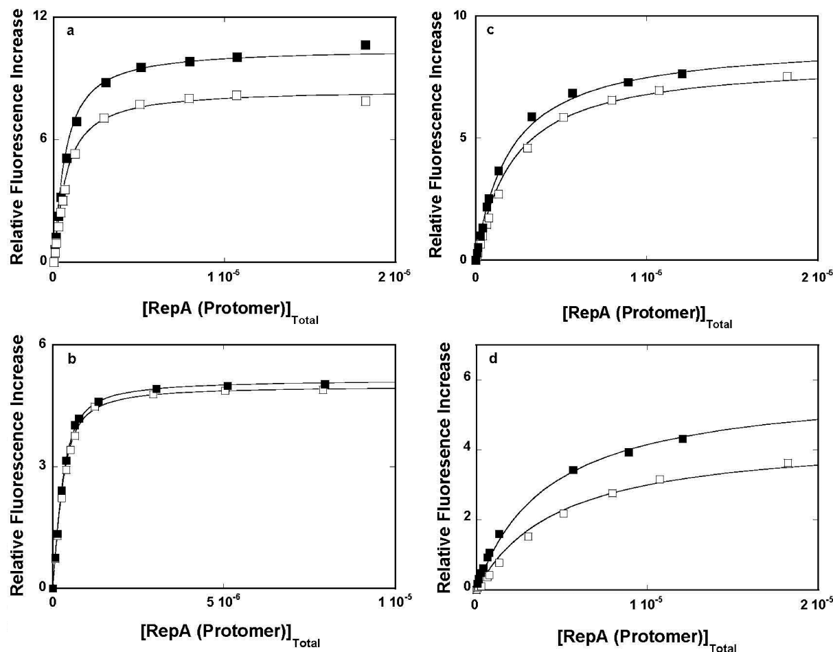
FIGURE 1: (a) Fluorescence titrations ( \lambda_{\text{ex}} = 410 nm, and \lambda_{\text{em}} = 560 nm) of TNP-ATP with the RepA helicase in buffer T5, containing 5 mM \text{MgCl}_2 , at 10 ( \square ) and 20 ^{\circ}\text{C} ( \blacksquare ). (b) Fluorescence titrations of TNP-ADP with the RepA helicase in buffer T5, containing 5 mM \text{MgCl}_2 , at 10 ( \square ) and 20 ^{\circ}\text{C} ( \blacksquare ). (c) Fluorescence titrations of TNP-ATP with the RepA helicase in buffer T5, in the absence of magnesium, at 10 ( \square ) and 20 ^{\circ}\text{C} ( \blacksquare ). (d) Fluorescence titrations of TNP-ADP with the RepA helicase in buffer T5, in the absence of magnesium, at 10 ( \square ) and 20 ^{\circ}\text{C} ( \blacksquare ). The solid lines in all panels are the nonlinear least-squares fits of the experimental titration curves to a single-site isotherm (eq 4) with the binding constant K_{\text{ov}} and the maximum relative fluorescence change, \Delta F_{\text{max}} , as fitting parameters. The concentrations of the nucleotide cofactors are 3 \times 10^{-7} M. The concentration of the RepA hexamer is expressed as protein protomers. The obtained binding constants and spectroscopic parameters are included in Tables 1 and 2.
