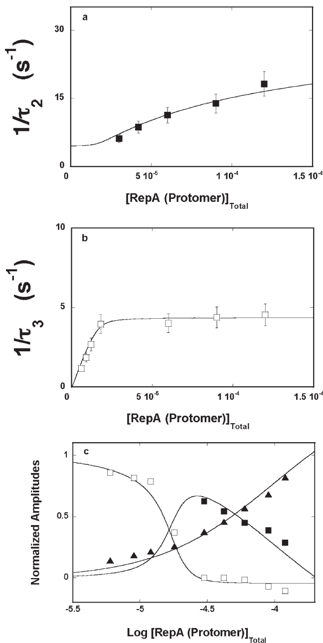
FIGURE 3: Dependence of the reciprocal relaxation times for the binding of TNP-ATP to the RepA helicase in buffer T5 (10 °C), containing 5 mM \text{MgCl}_2 , on the total concentration of the enzyme (protomer): (a) 1/\tau_2 (■) and (b) 1/\tau_3 (□). (c) Dependence of the individual normalized relaxation amplitudes A_1 (▲), A_2 (■), and A_3 (□), of the kinetic process of binding of TNP-ATP to the RepA helicase in buffer T5 (10 °C), containing 5 mM \text{MgCl}_2 , on the logarithm of the total concentration of the enzyme (protomer). The solid lines in panels a, b, and c are nonlinear least-squares fits of the experimental data to the three-step sequential mechanism, defined by eq 5. The obtained kinetic and spectroscopic parameters are included in Table 1 (details in the text). The error bars are standard deviations obtained from three or four independent experiments.
